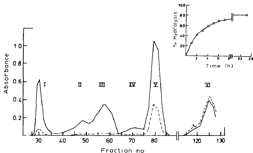
Fig. 1. Gel filtration of a 6-h pronase digest of Tamm-Horsfall glycoprotein (26 mg) on a column (110 \times 2.2 cm) of Sephadex G25 (fine) in 0.1M acetic acid (fraction volume, 5.4 mL): glycopeptides (I), other u.v.-absorbing materials (II–VI); absorbances at 280 (----) and 230 nm (—) are shown. The inset illustrates the rate of proteolysis, catalysed by pronase, of Tamm-Horsfall glycoprotein (see Experimental).
