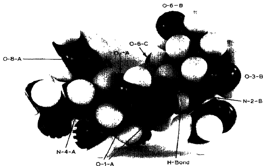
Fig. 4. A molecular model of the trisaccharide terminal unit \alpha -NeuAc-(2 \rightarrow 3)[ \beta -GalNAc-(1 \rightarrow 4)]-Gal-. Pertinent atoms are identified, with A, B, and C referring to NeuAc, GalNAc, and Gal residues, respectively.
